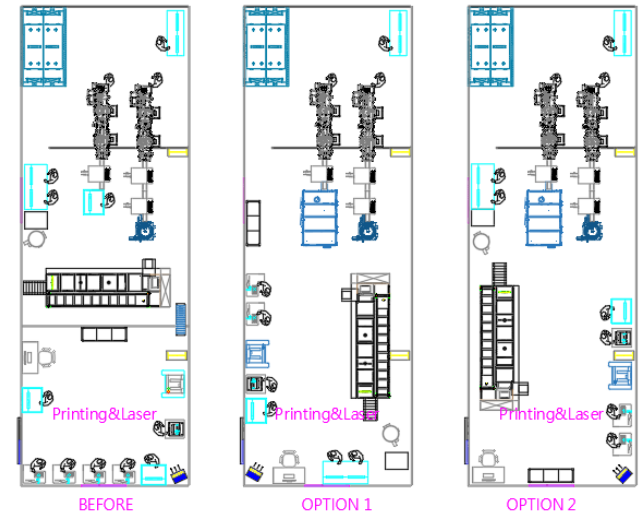
Laser area layout
